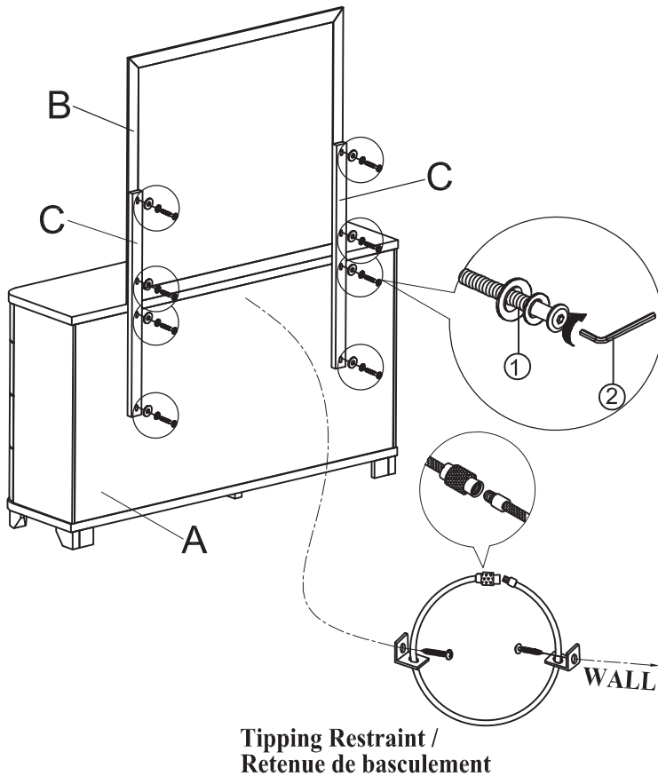
COMPLETED DRESSER & MIRROR ASSEMBLY
