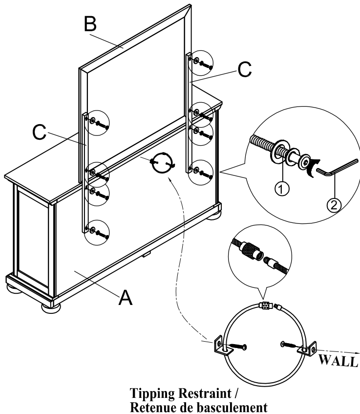
COMPLETED DRESSER & MIRROR ASSEMBLY
