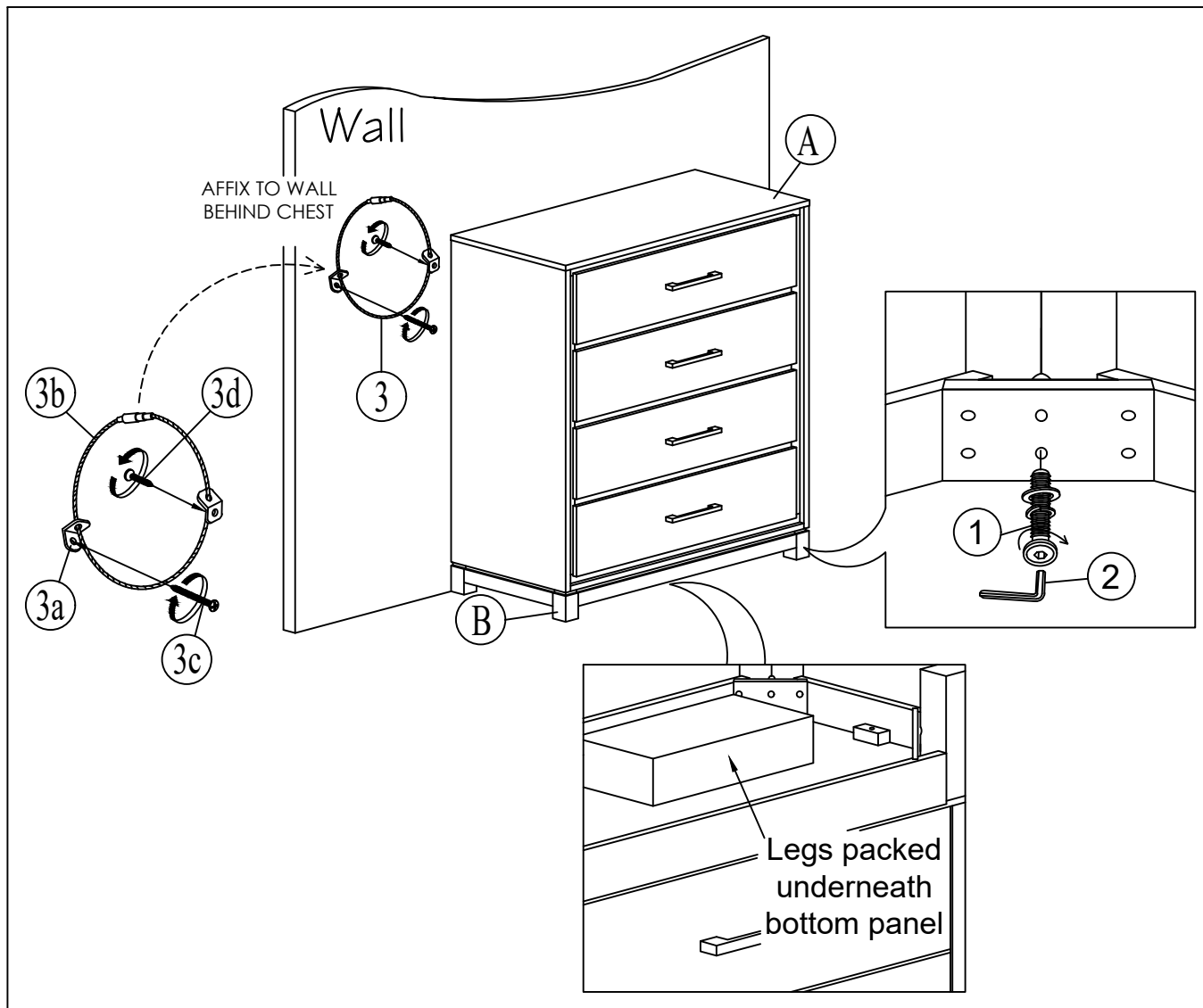
COMPLETED CHEST ASSEMBLY
