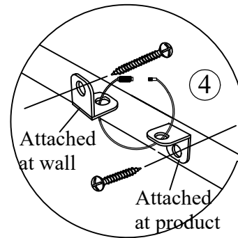
Anti - Tip Kit
